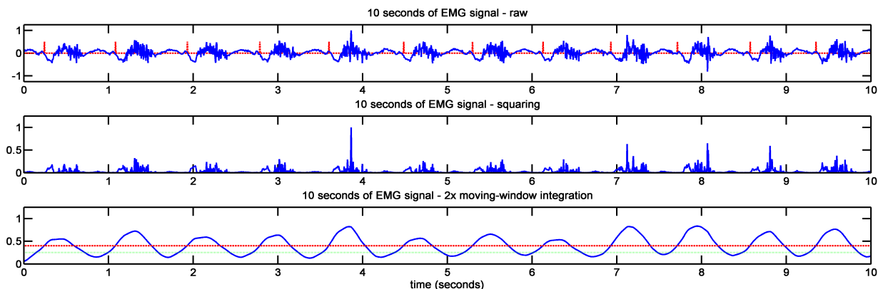
Fig. 2. Processing pipeline for the EMG signal. In this figure, 10 seconds of the signal were extracted for the processing. From top to bottom: (1) raw EMG signal (blue, solid), detected treadles by the algorithm (red, dashed); (2) signal after squaring operation, (3) signal after double moving-window integration (blue, solid), threshold (red, dashed), minimum threshold for avoiding misdetection (green, dotted).
