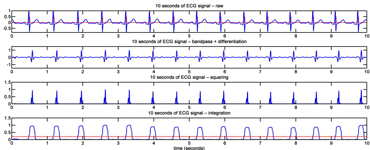
Fig. 1. Processing pipeline for the ECG signal. In this figure, 10 seconds of the signal were extracted for the processing. From top to bottom: (1) raw ECG signal (blue, solid), detected heart beats by the algorithm (red, dashed); (2) signal after bandpass filter and differentiation, (3) signal after squaring operation; (4) signal after moving-window integration (blue, solid), threshold (red, dashed).
